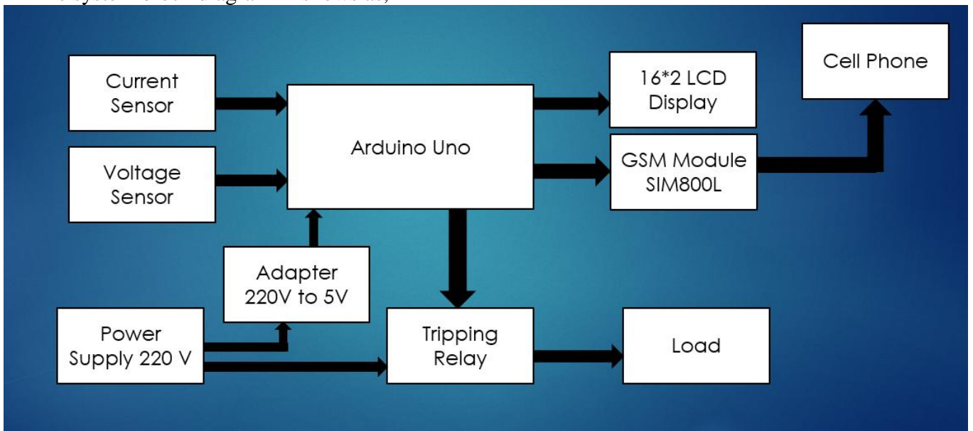
Fig. 2.3 System block diagram
