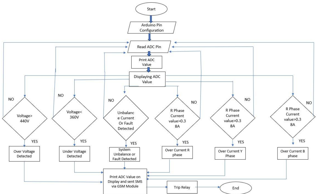
Fig. 3.1 Flowchart of this project
