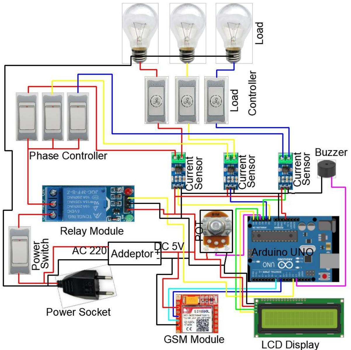
Fig.3.2 Circuit diagram of this project
