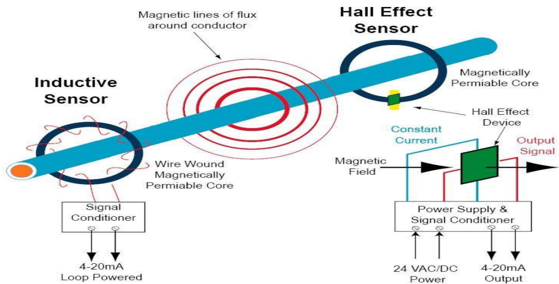
Fig. 2.2 Working principle of current sensor
