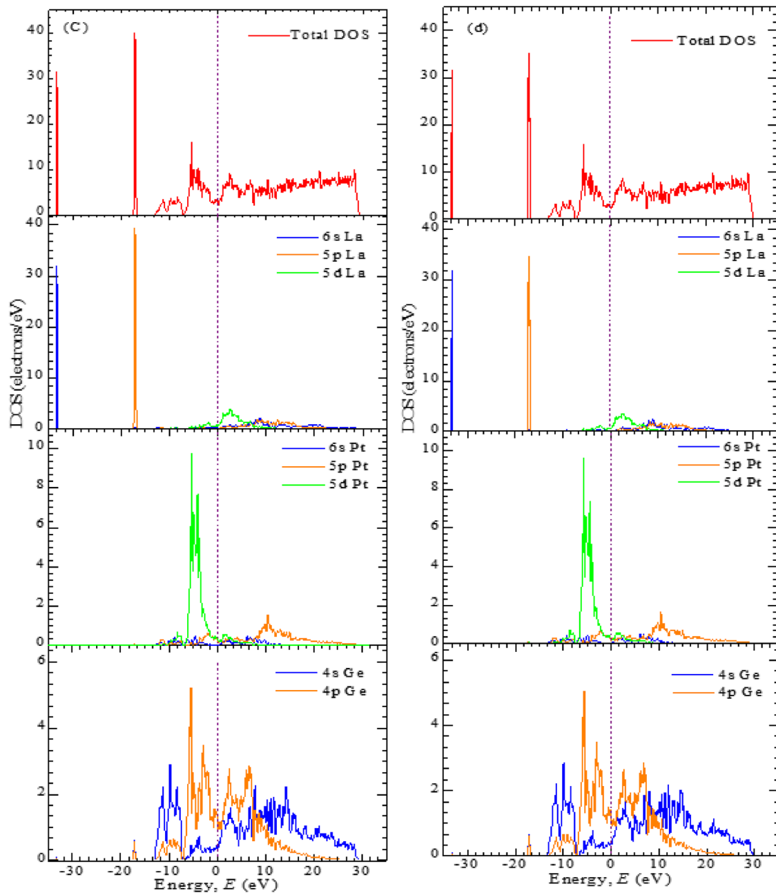
FIG. 5. Total and partial density of states (DOS) of \text{LaPtGe}_3 at (c) P = 10 GPa and (d) P = 15 GPa.
