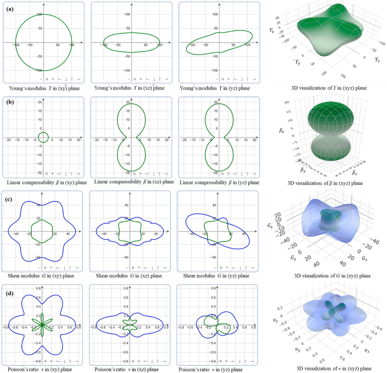
Fig. 3. Directional anisotropy (2D and 3D) of (a) Young's modulus (b) compressibility (c) shear modulus and (d) Poisson's ratio for \text{Ti}_2\text{PTe}_2 .
