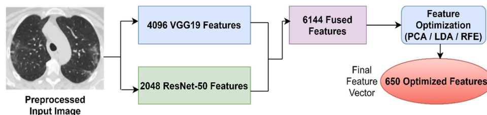
Fig. 5. Feature minimization process of this research.
