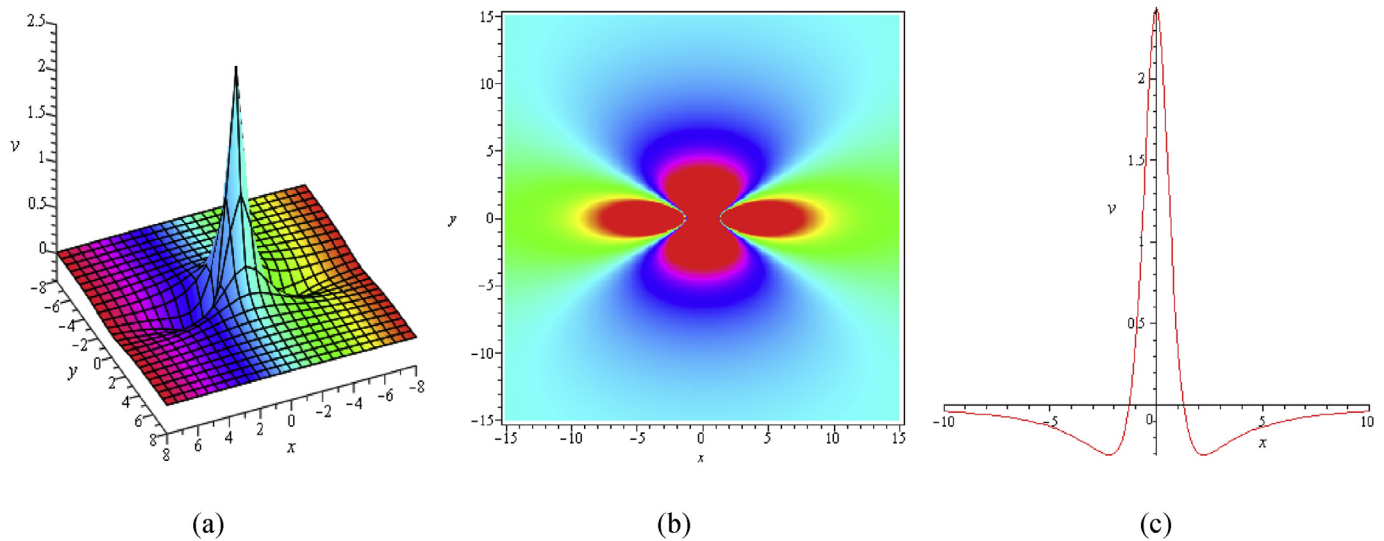
Fig. 7. Lump solution v in (20) for Eq. (1) by choosing suitable parameters: p_1 = 2 , l_2 = 1 , m_1 = 2 , and m_2 = 1 . (a) 3-D plot of v (b) density plot of v (c) 2-D plot of v .
