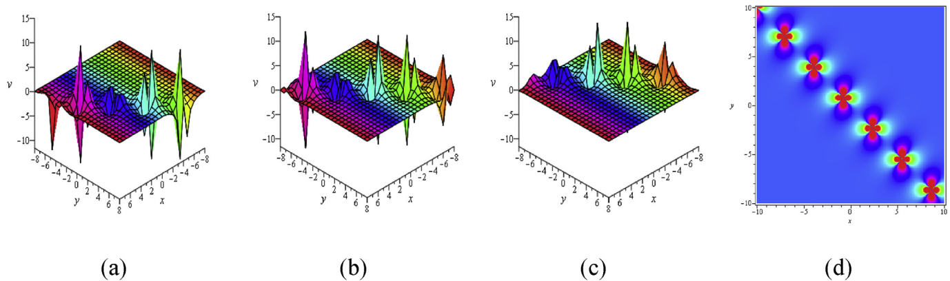
Fig. 10. Profiles of v in (35) with t = -2, 0, 2 : 3d plots (a), (b), (c) respectively and (d) corresponding density plot (b) by choosing suitable parameters: h_1 = 1 , h_2 = 2 , p_1 = 1 , p_2 = -1 and n_2 = -1 .
