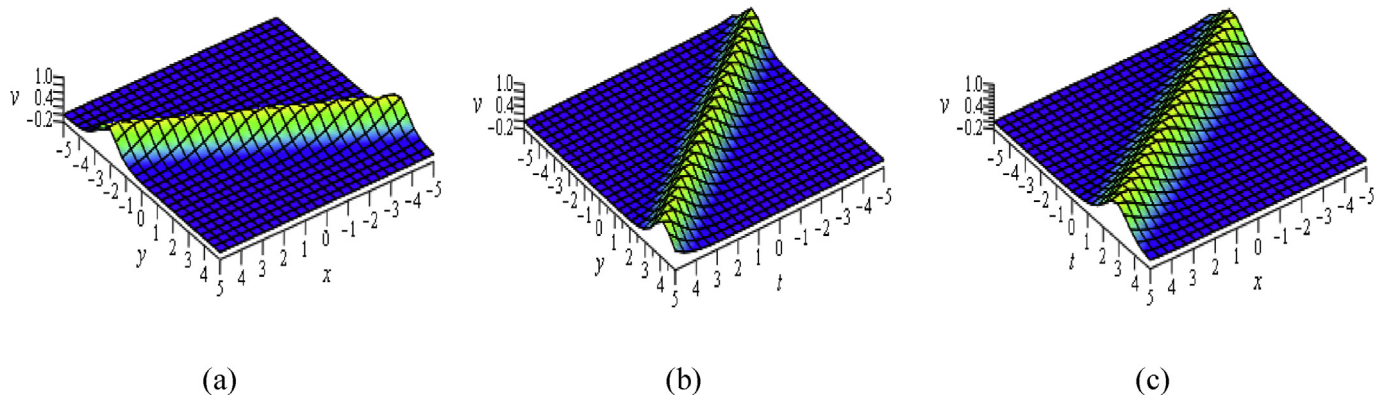
Fig. 1. The one-stripe soliton solution for Eq. (1) by choosing suitable parameters: a_0 = 2, a_1 = 1, l_1 = 1.25, m_1 = 2.5 , 3D shape in different planes at (a) t = 0 ; (b) x = 0 ; and (c) y = 0 .
