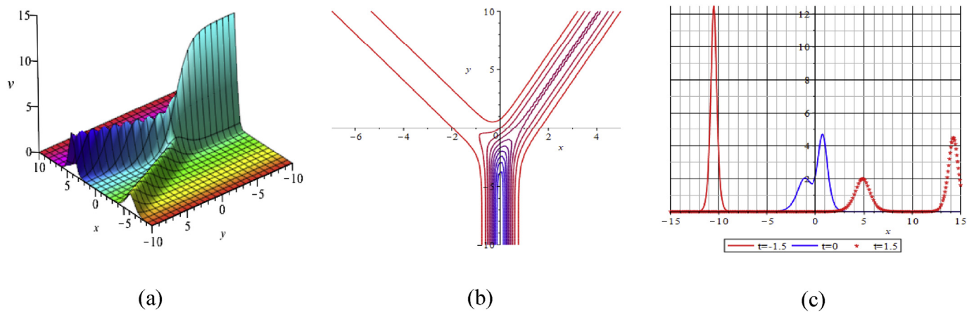
Fig. 3. The two-stripe soliton solution (non-elastic) for Eq. (1) by choosing suitable parameters: a_1 = 1 , a_2 = 1 , a_3 = 10 , l_1 = 2 , l_2 = -3 , m_1 = m_2 = 1 , at time t = 0 (a) 3D plot (b) Contour plot and (c) Corresponding 2D plot for different time.
