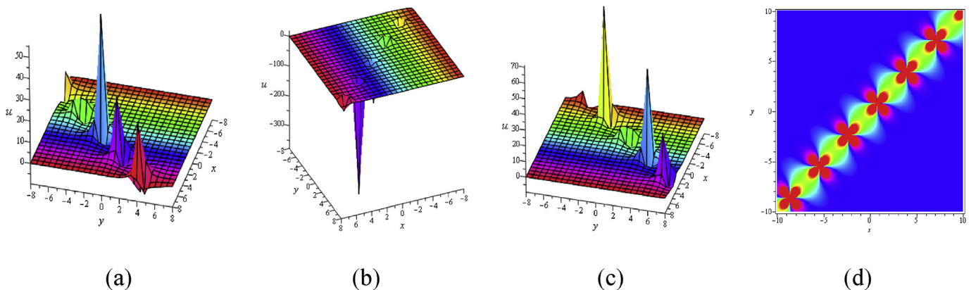
Fig. 9. Profiles of u in (34) with t = -1.5, 0, 1.5 : 3d plots (a), (b), (c) respectively and (d) corresponding density plot (b) by choosing suitable parameters: h_1 = 1 , h_2 = 2 , p_1 = 1, p_2 = -1 and n_2 = 1 .
