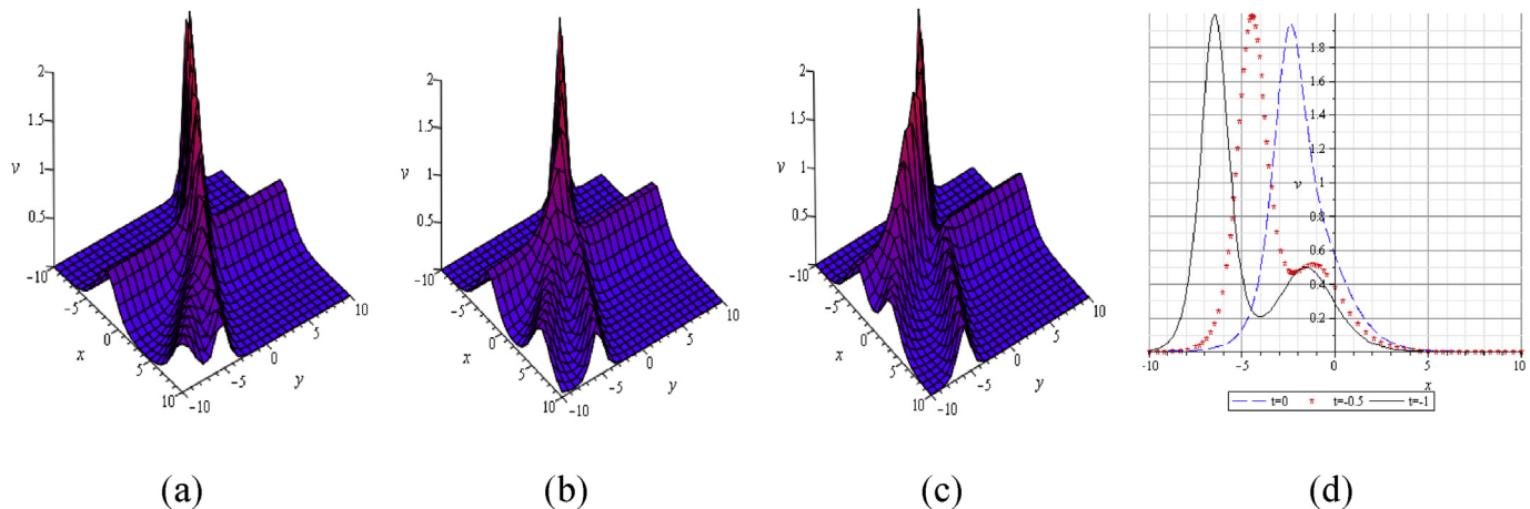
Fig. 5. The three-stripe soliton solution for Eq. (1) by choosing parameters: a_{13} = 2, l_1 = 1, l_2 = 2, l_3 = 2, m_2 = 1, m_3 = 3 , with 3D plots at (a) t = 0 , (b) t = -0.5 , and (c) t = -1 respectively, (d) 2D plot at t = 0, -0.5 and t = -1 respectively.
