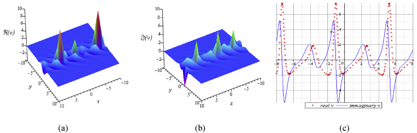
Fig. 4. The breather solution for Eq. (1) by choosing suitable parameters: a_1 = 1 , a_2 = 1 , a_3 = 10 , l_1 = 2 , l_2 = 2.5 , m_1 = 1 , m_2 = 3.5 , with t = 0 : 3D plots (a), (b) and (c) Corresponding 2D plot.
