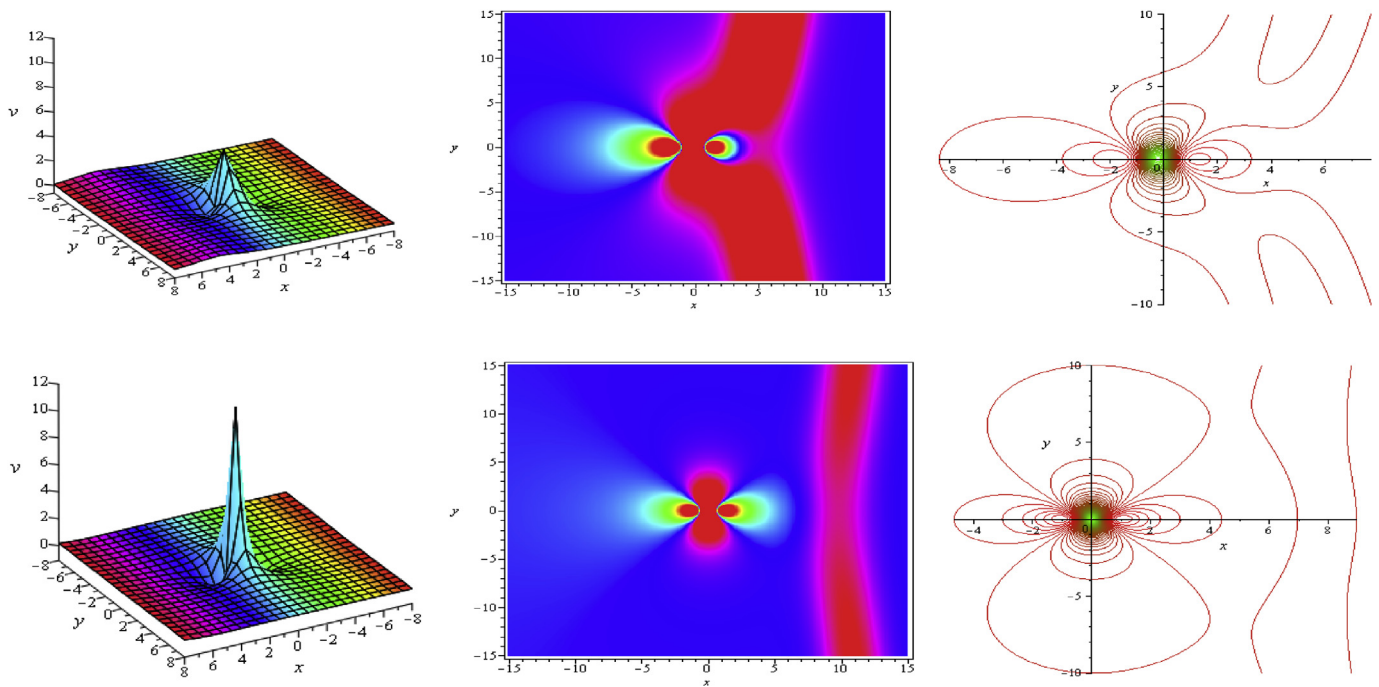
Fig. 8. Profiles of v in (29) with t = 0 : 3d plots, density plot and contour plot (top for a_2 = 5 ) and bottom for a_2 = 0.05 by choosing suitable parameters: a_1 = 2.5 , m_1 = 2.3 , m_2 = 1 , l_1 = 1.5 , and l_3 = 1 .
