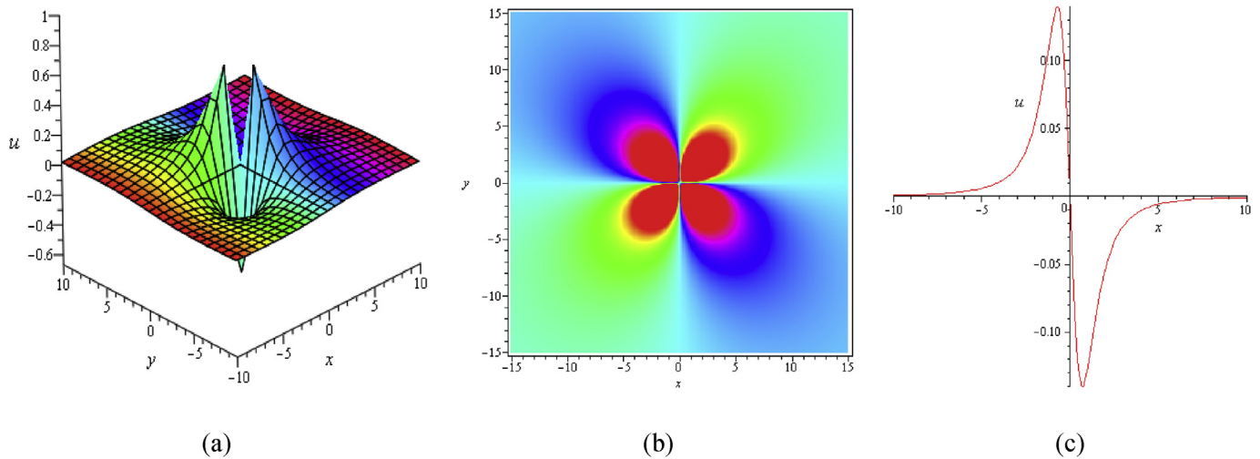
Fig. 6. Lump solution u in (20) Eq. (1) by choosing suitable parameters: p_1 = 1.2 , l_2 = 0.8 , m_1 = -0.8 , and m_2 = 0.4 (a) 3-D plot of u (b) density plot of u (c) 2-D plot of u .
