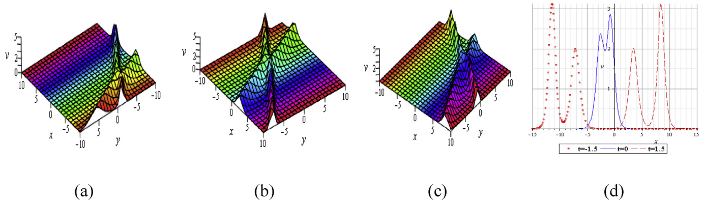
Fig. 2. The two-stripe soliton solution for Eq. (1) by choosing suitable parameters: a_1 = 1 , a_2 = 1 , a_3 = 10 , l_1 = 2 , l_2 = 2.5 , m_1 = 1 , m_2 = 3.5 , with 3D plots for different times (a) t = -1.5 ; (b) t = 0 ; and (c) t = 1.5 respectively, (d) Corresponding 2D plot.
