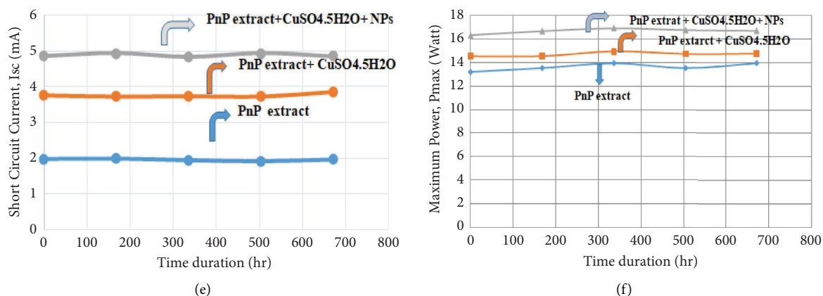
FIGURE 11: The influence of AgNPs on three distinct scenarios in the bioelectrochemical cell, utilizing PgP and PnP extracts: (a) open-circuit voltage for PgP, (b) short-circuit current for PgP, (c) maximum power for PgP, (d) open-circuit voltage for PnP, (e) short-circuit current for PnP, and (f) maximum power for PnP.
