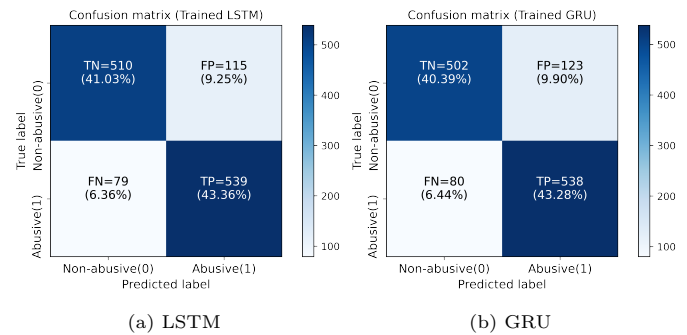
Fig. 12. Confusion Matrix of LSTM and GRU Classifiers on Trained Word Embedding Feature Extraction.
