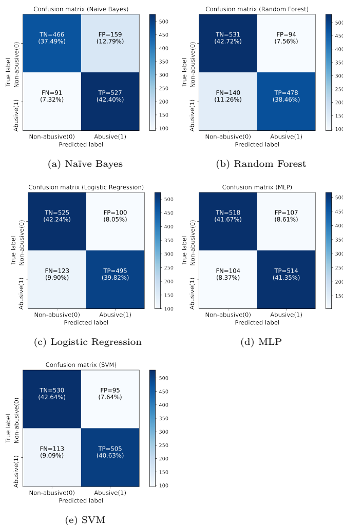
Fig. 11. Confusion Matrix of Traditional Classifiers on n-gram TF-IDF Feature Method.
