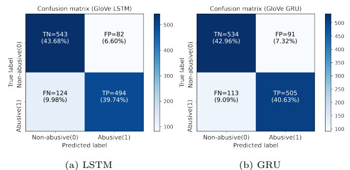
Fig. 13. Confusion Matrix of LSTM and GRU Classifiers on Pre-trained GloVe Embeddings Model.
