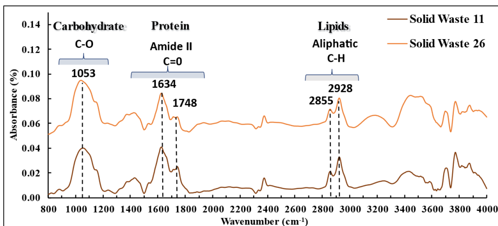
Figure 4. FTIR analysis of solid waste biomass
