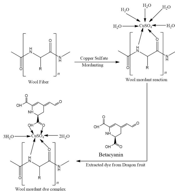
Figure 5. Complex reaction mechanism of wool–copper sulfate mordant for natural dye extracted from dragon fruit.
