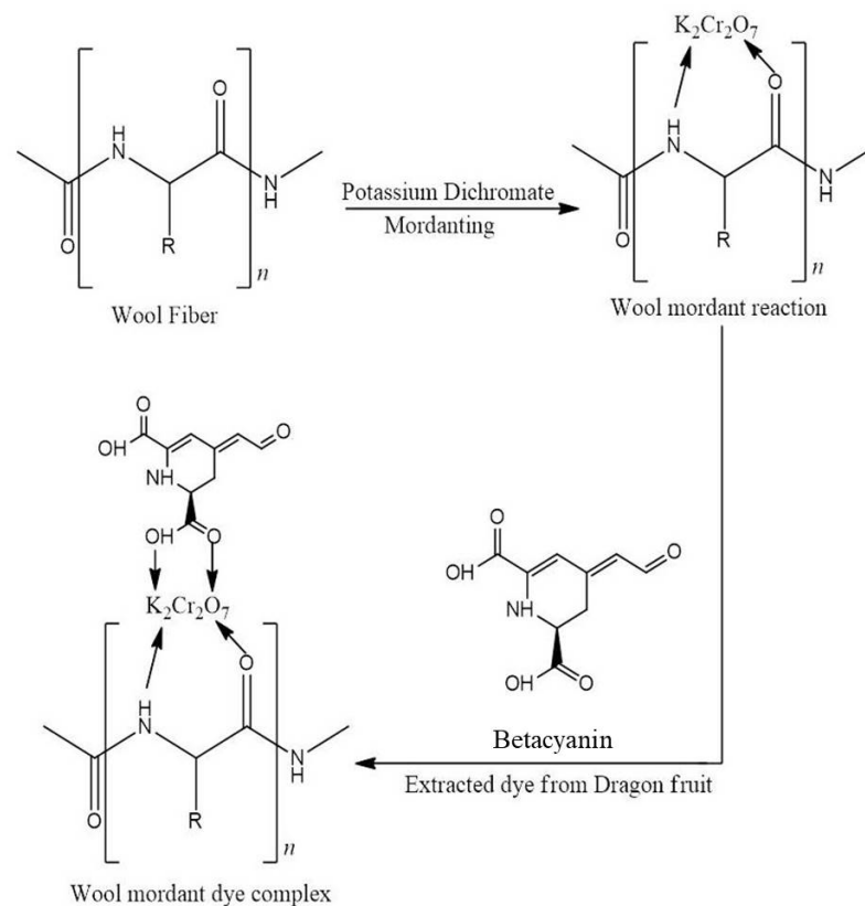
Figure 4. Complex reaction mechanism of wool–potassium dichromate mordant for extracted natural dye from dragon fruit.
