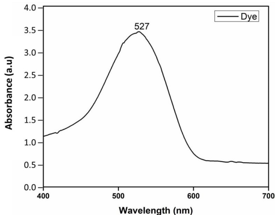
Figure 8. Dye absorption spectrum of dragon fruit dye in the range of 400 nm to 700 nm.
