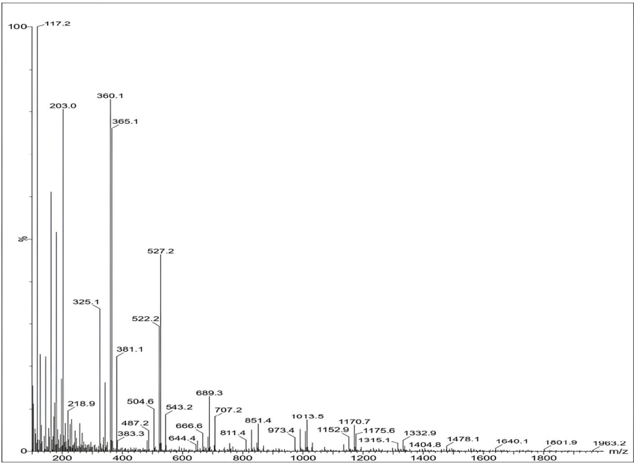
Figure 10. Mass spectra of degraded compounds.
