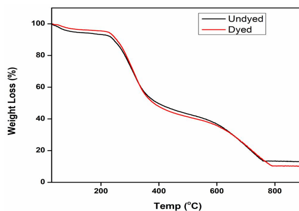
Figure 7. TGA curves of undyed and dyed wool fabric with dragon fruit extract.
