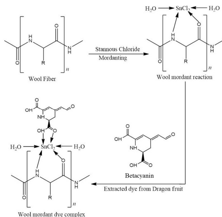
Figure 6. Complex reaction mechanism of wool–stannous chloride mordant for natural dye extracted from dragon fruit.
