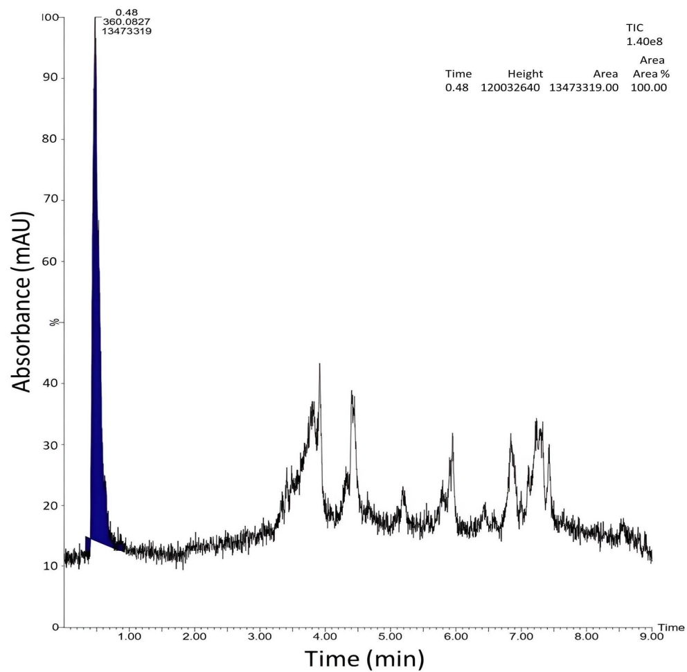
Figure 9. Chromatogram of dragon fruit dye.
