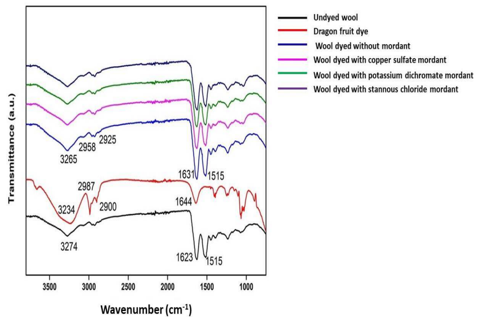
Figure 3. FTIR spectra of raw wool, natural dye extracted from dragon fruit, wool dyed without mordant, wool dyed with copper sulfate mordant, wool dyed with potassium dichromate mordant, and wool dyed with tin chloride mordant.
