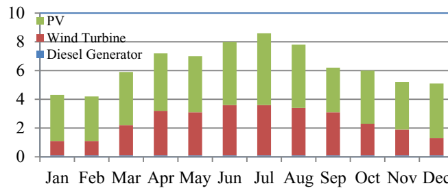
Fig. 8. Energy generated with practicability from the smart-grid hybrid PV-wind-diesel-battery energy system.
