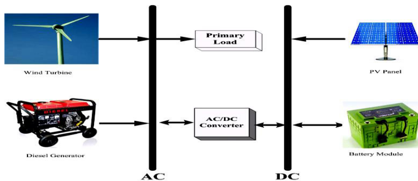
Fig. 7. Schematic diagram of a hybrid energy system.
