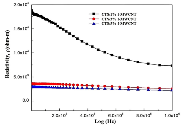
FIGURE 10 Variation of resistivity ( \rho ) with frequency ( \log f ) for CTS/1% f-MWCNTs, CTS/3% f-MWCNTs, and CTS/5% f-MWCNTs composites. CTS, chitosan; MWCNTs, multi-walled carbon nanotubes.
