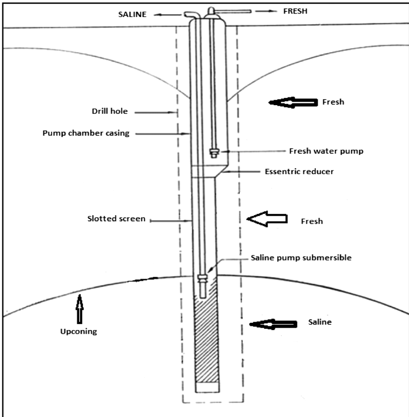
Fig. 3. Schematic diagram of scavenger well.
