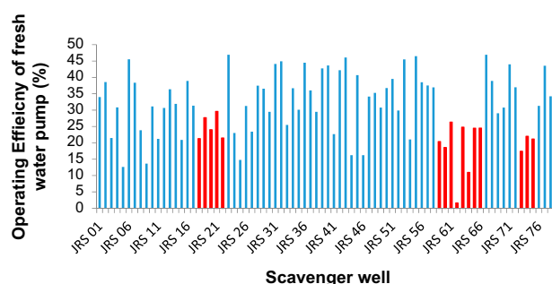
Fig. 10. Operational efficiency of fresh water pump of scavenger wells.
