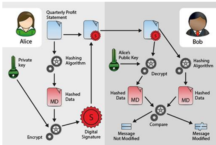
Fig. 4. Illustration of the digital signature process
